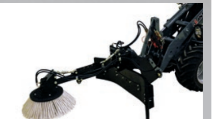
FEED AND MANURE SCRAPER WITH BRUSH HYDRAULICALLY GA300
